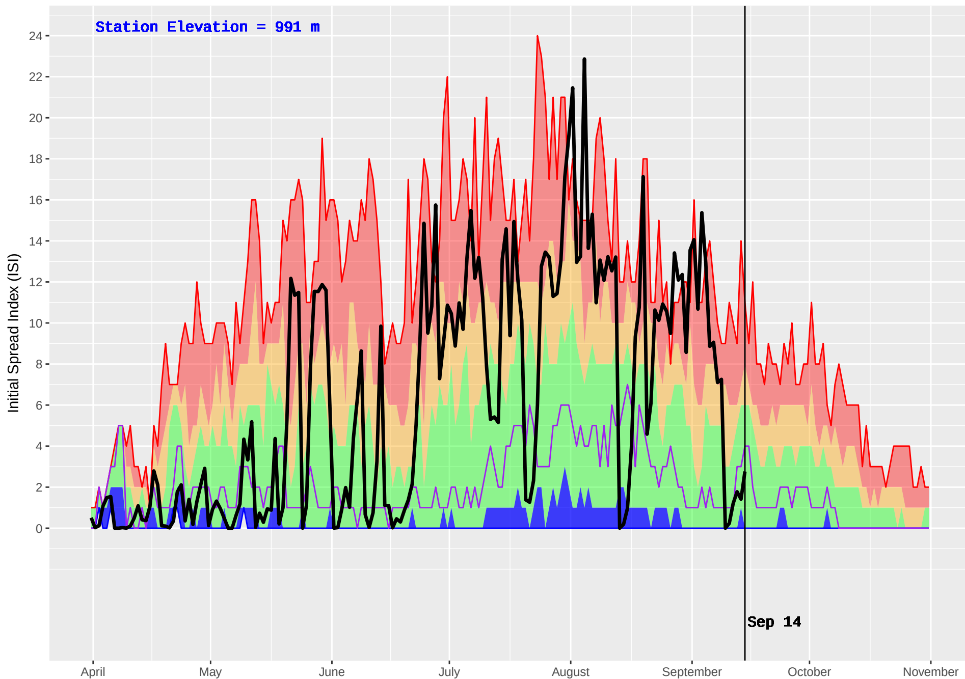
TROUT LAKE (387) : Historical (1987–2016) and Current (2017) Noon Initial Spread Index (ISI)
