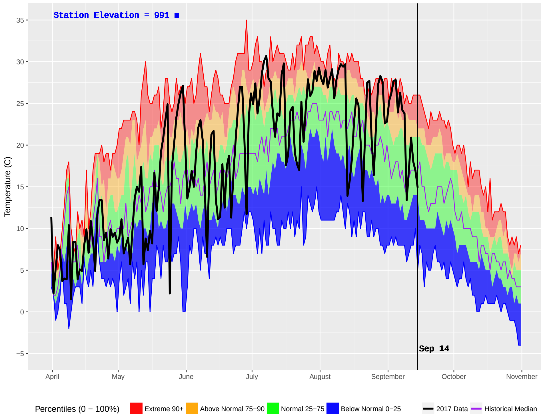
TROUT LAKE (387) : Historical (1987–2016) and Current (2017) Noon Temperature
